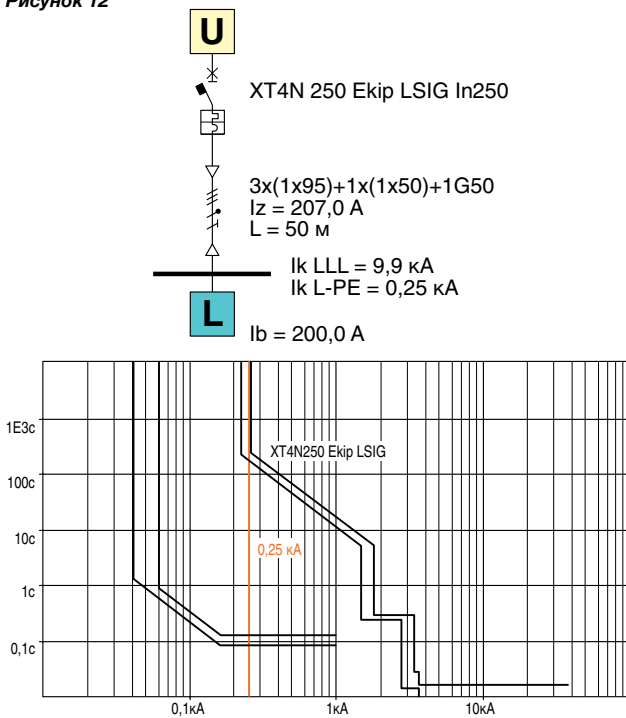
XT4N 250 Ekip LSIG In 250 A
