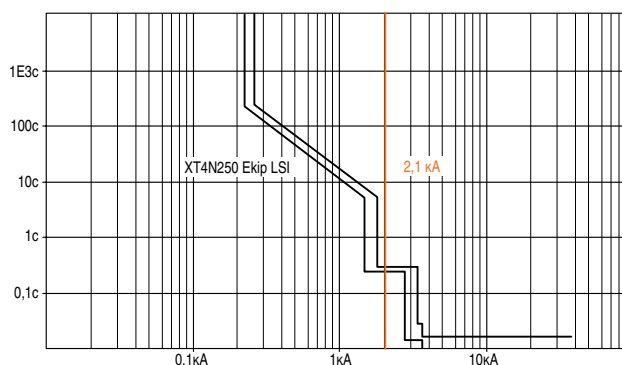
XT4N 250 Ekip LSI In 250 A
